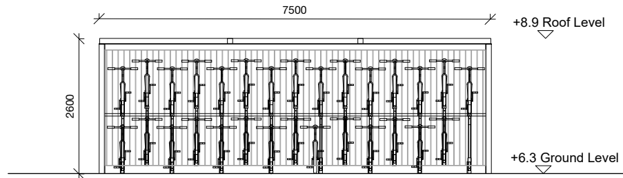
Section
